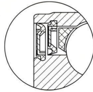
密封型式4RS Seal Type 4RS
