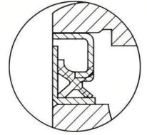
密封型式ZZ Seal Type ZZ
